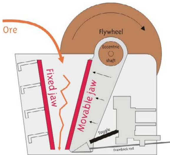
Jaw crushers handle large blocks of ore and are the primary crushing stage.
