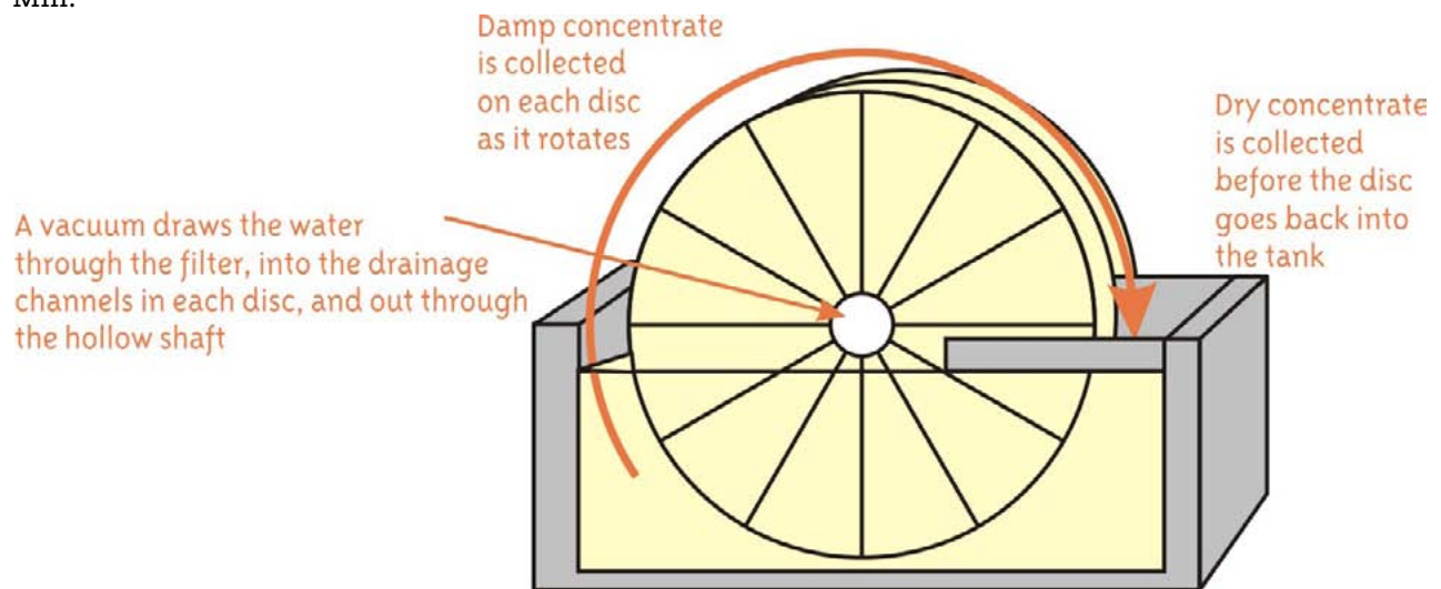
Disc filters were the last stage of concentrate production, drying it before shipment to smelter
